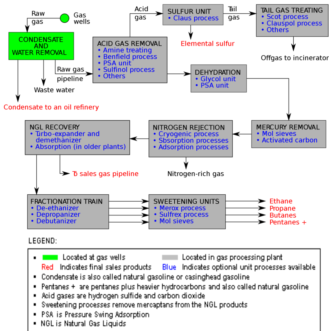
Fig. 1: Schematic Flow Diagram of a Typical Natural Gas Processing Plant
