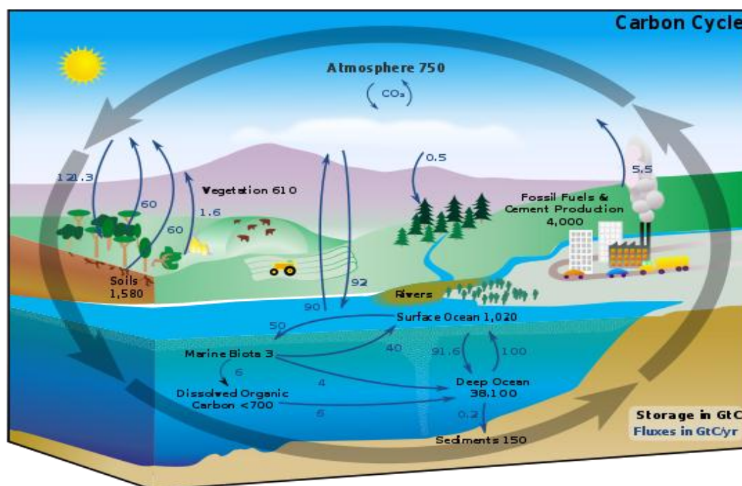
Fig. 3 : Diagram of the Carbon Cycle
