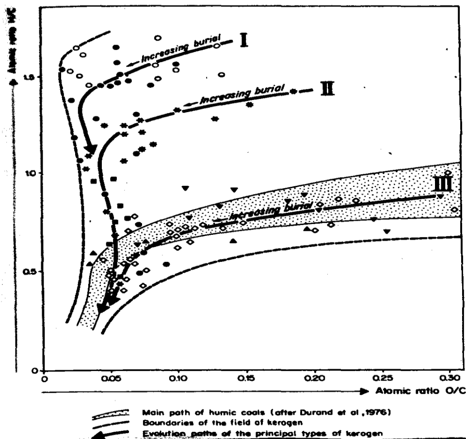
Fig. 1 : Van Krevelen Diagram (Principal types and evolution path of kerogen: types I, II and III are most frequent. Kerogen of intermediate composition also occurs. Evolution of kerogen composition with increasing burial is marked by an arrow along each evolution path I, II, and III
