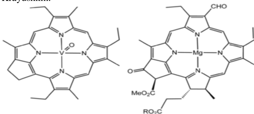
Fig. 2: Structure of Vanadium porphyrin compound (left) extracted from petroleum by Alfred Treibs, father of organic geochemistry. Treibs noted the close structural similarity of this molecule and chlorophyll (right)
